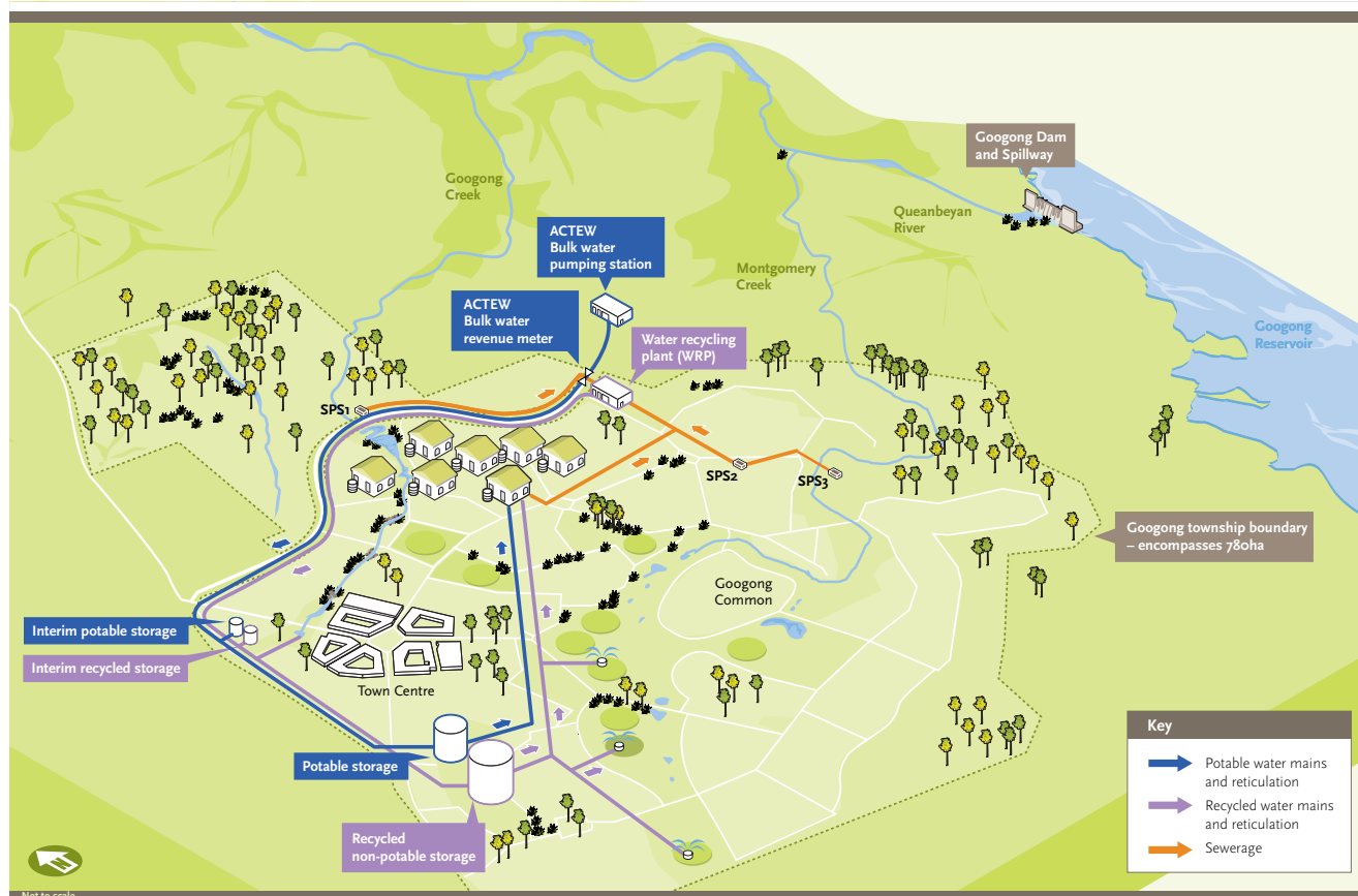
Figure 1. Googong Integrated Water Cycle Schematics
